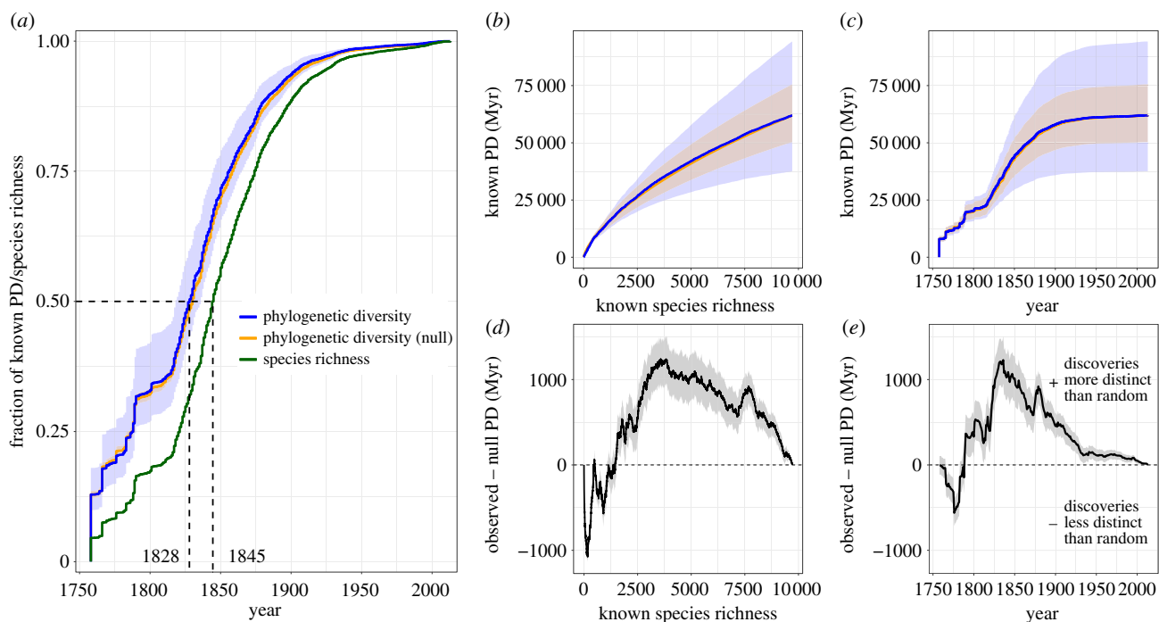
Figure 1. Accumulation of known PD and species richness in birds. (a) Cumulative fraction of present-day known PD (blue/orange) or species richness (green) discovered over the period of modern taxonomy. The dotted lines indicate when half of present-day PD or species richness had been discovered. (b–c) The accumulation of known PD over successive species discoveries (b) and over time (c). (d–e) The difference between the blue and orange lines in (b) and (c), respectively. In all figures, the orange line shows the known PD accumulation when the discovery order is randomized (i.e. the null model). Shaded areas indicate the 95% confidence intervals for known PD. (Online version in colour.)
